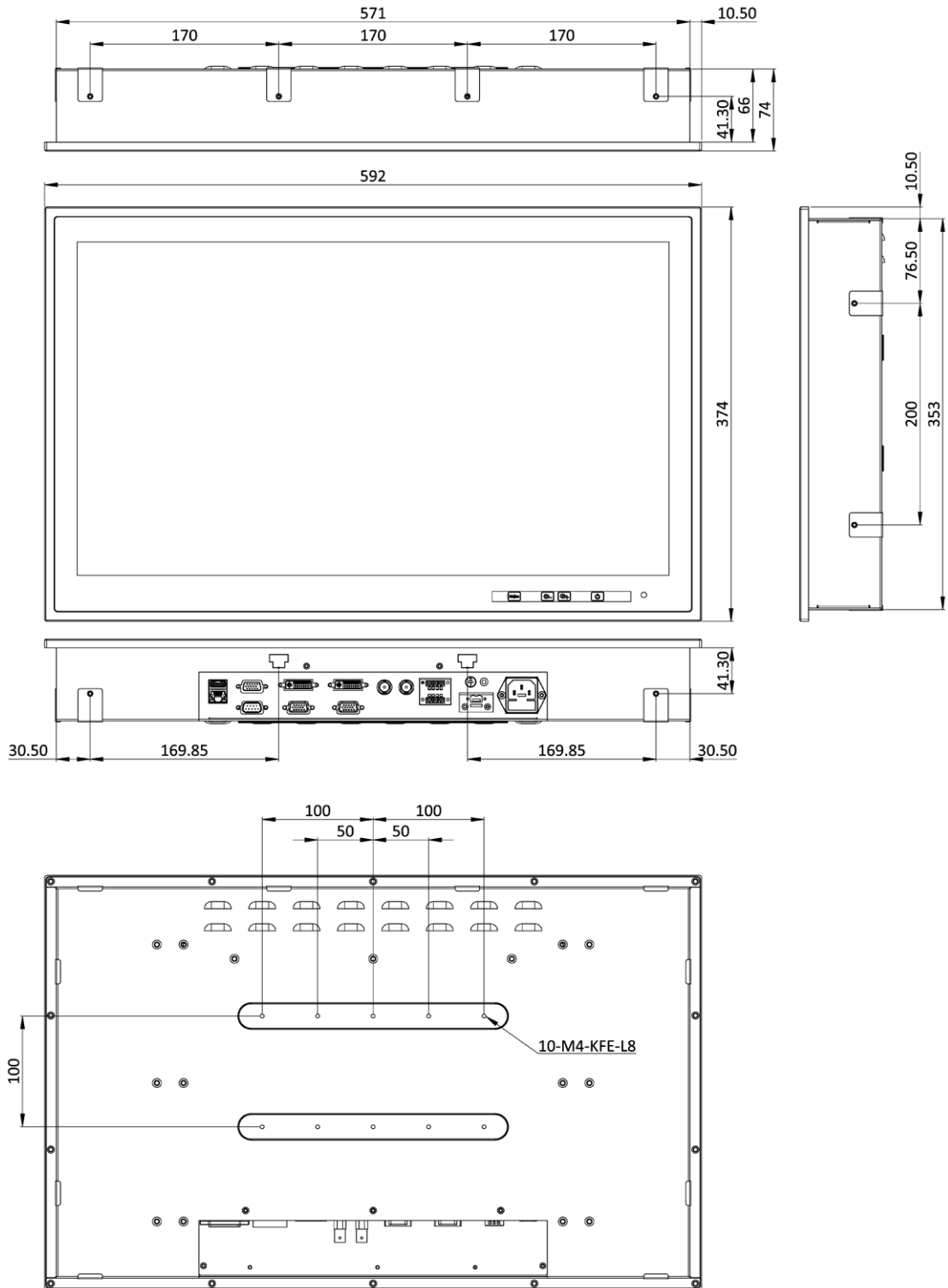
Figure 1-8: S24M Dimensions (mm)
