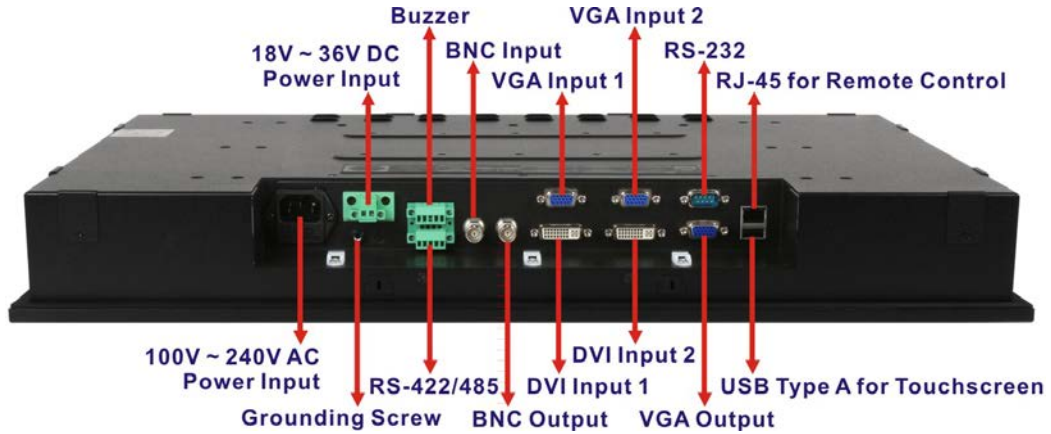
Figure 3-5: I/O Interfaces
