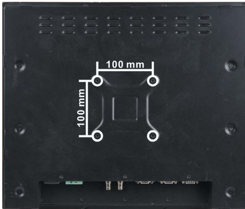
Figure 1-5: S19M Rear Panel
