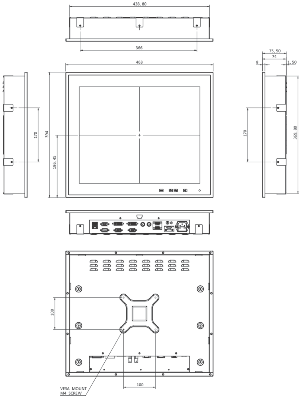
Figure 1-7: S19M Dimensions (mm)
