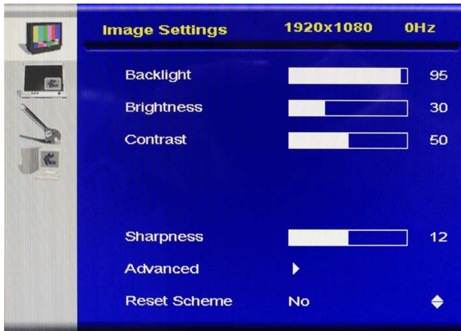
Figure 4-2: Main Menu
