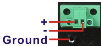
Figure 3-6: 18V ~ 36V DC Power Input Terminal Block Pinouts
