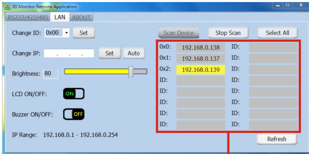
Device List
