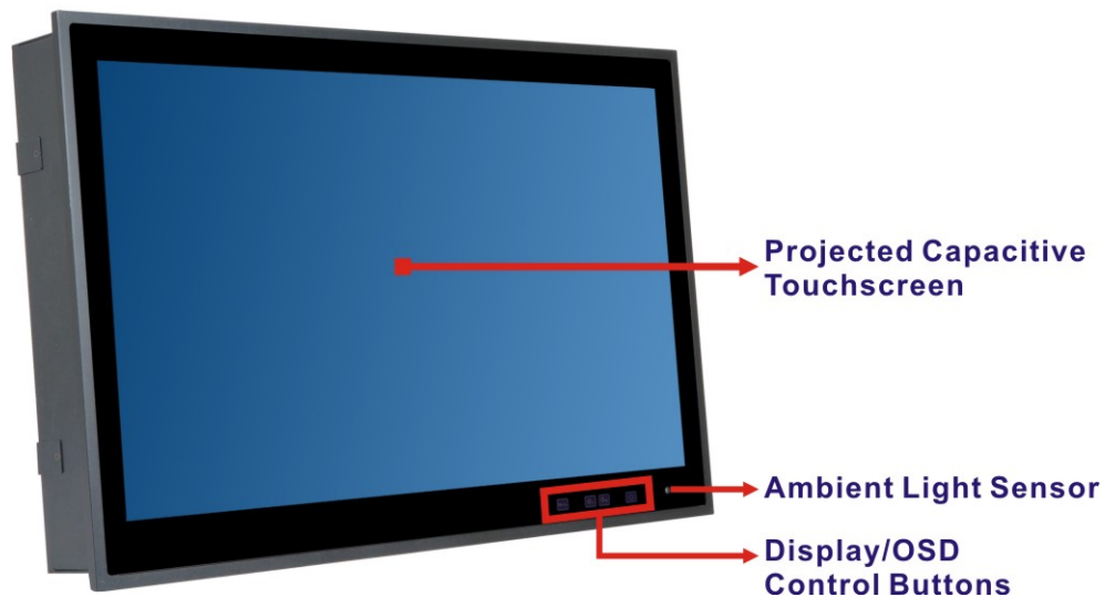
Figure 1-2: Front Panel
