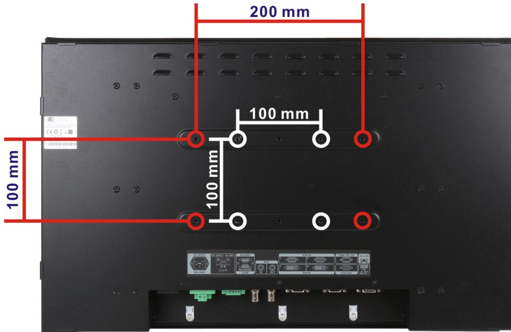
Figure 1-6: S24M Rear Panel
