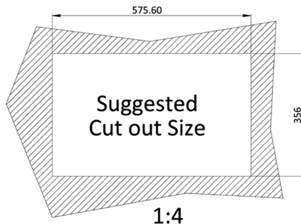
Figure 3-2: S24M Cutout Dimensions
